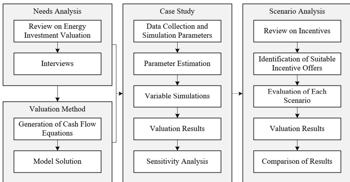
Fig. 1. Research methodology.
