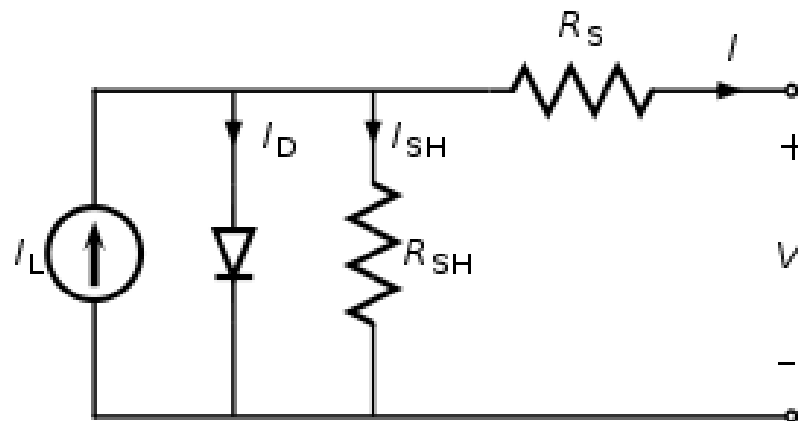
Figure 2.6: The equivalent circuit of PV cell
