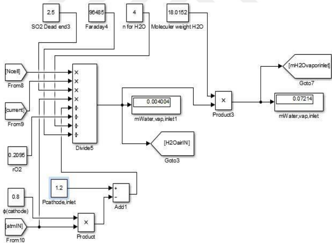
Figure 4.11: The inlet mass flowrate amount of water vapor in air calculation by PEMFC in Simulink block diagram
