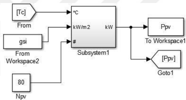
Figure 4.1: The power calculation of PV arrays in Simulink block diagram
