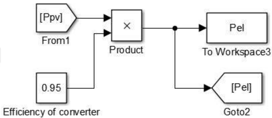
Figure 4.3: The power calculation of electrolyzer in Simulink block diagram
