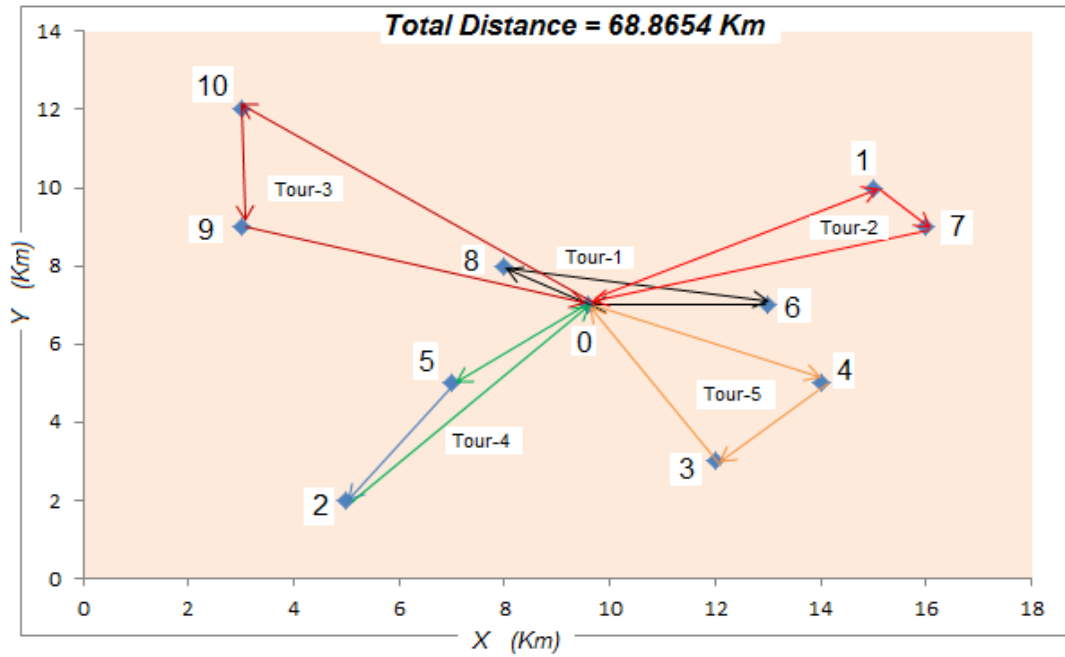
Figure 5.7: The tours obtained by ACOA for the drone with 10 customers, location 0 represents the delivery truck.
