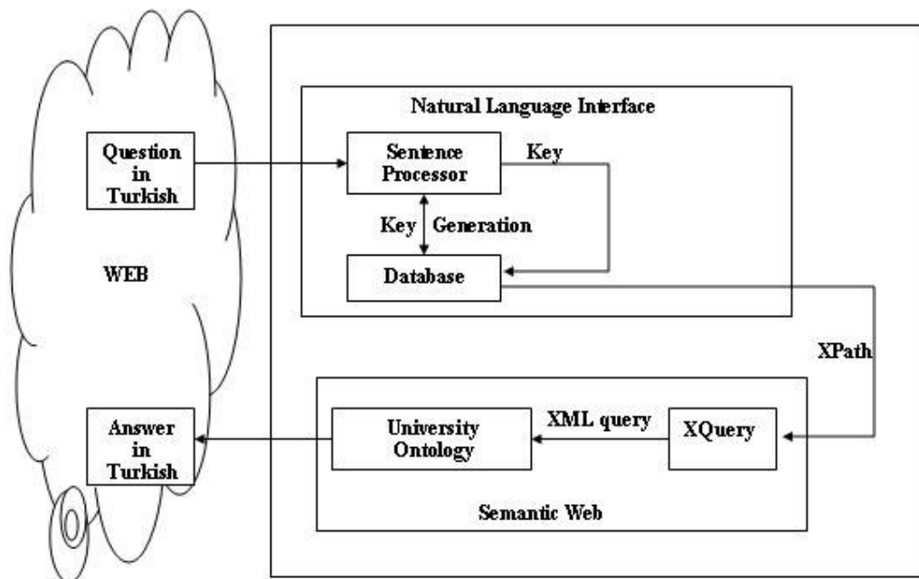
Figure 4.1 Components of the System
