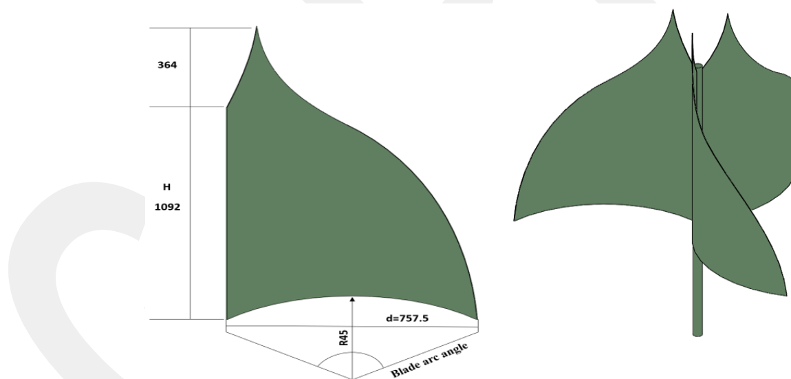
Figure 10. IceWind blade (dimensions in mm).
