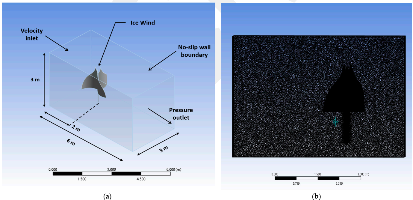
Figure 12. IceWind model in ANSYS: (a) IceWind turbine and domain dimensions (m); (b) mesh of the IceWind turbine domain from side view.
